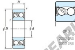
Spherical Ball Bearings Sealed type Sealed type All
