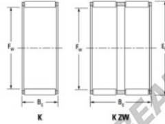
Rolls needle roller and cage assemblies
