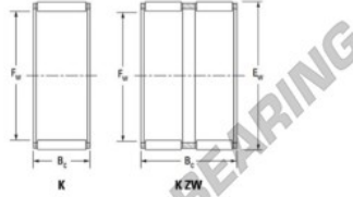
Boundary dimensions
