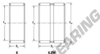
Partial Needle roller and cage assemblies
