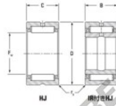
Boundary dimensions
