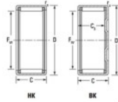
Boundary dimensions
