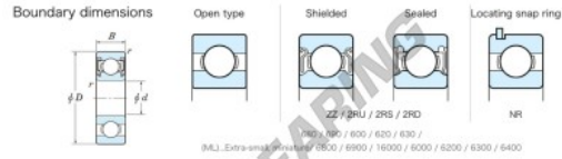
Extra-Small (rotating) non contact sealed 2RU
